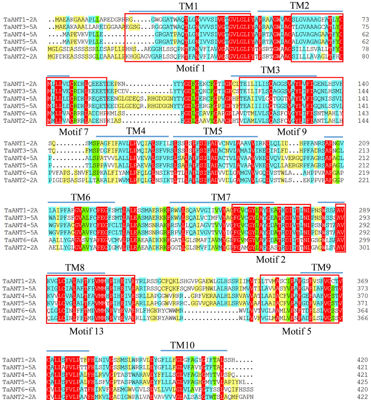
Fig. 6. Multiple sequence alignment of the transmembrane (TM) region of the aromatic and neutral amino acid transporter (ANT) subfamily members in wheat. The blue line represents the TM regions of TaANT proteins, and the red box represents the conserved motifs predicted by Multiple EM for Motif Elicitation (MEME). Identical (100%), conserved (75–99%), and blocks of similar (50–74%) amino acid residues are shaded in red, blue, and yellow, respectively.
